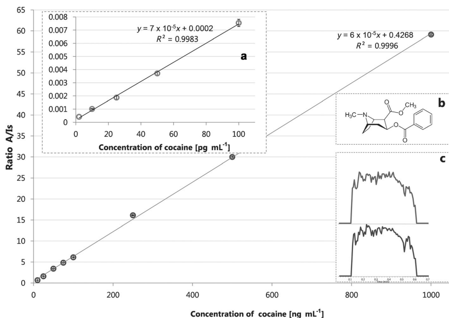
Figure 2. Quantitative analysis of PBS spiked with cocaine ( 2 \text{ pg mL}^{-1} to 1 \text{ } \mu\text{g mL}^{-1} ) and its isotopologue [D 3 ]cocaine ( 14.5 \text{ ng mL}^{-1} ). Bars represent the standard deviation of analyses for three replicates with independent blades. a) Plot showing the low-concentration range. b) Molecular structure of cocaine. c) Ion chromatogram of cocaine (top) and [D 3 ]cocaine (bottom) for an acquisition time of 30 s.
